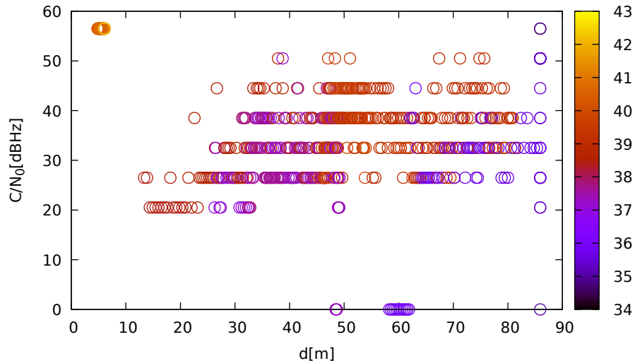
C/N 0 vs distance (LeicaGS15 at C 3 for G32 at L1)
