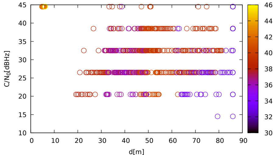
C/N 0 vs distance (LeicaGS15 at C 3 for R06 at L1)
