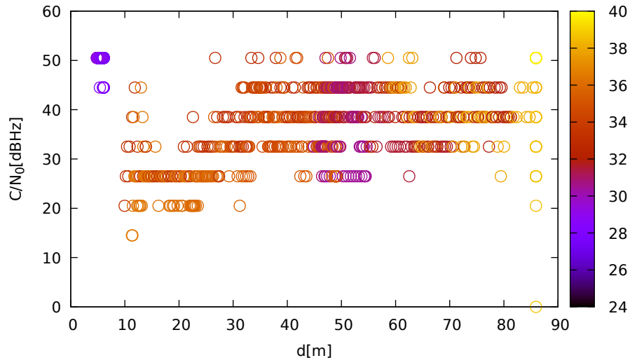
C/N 0 vs distance (LeicaGS15 at C 3 for R08 at L1)
