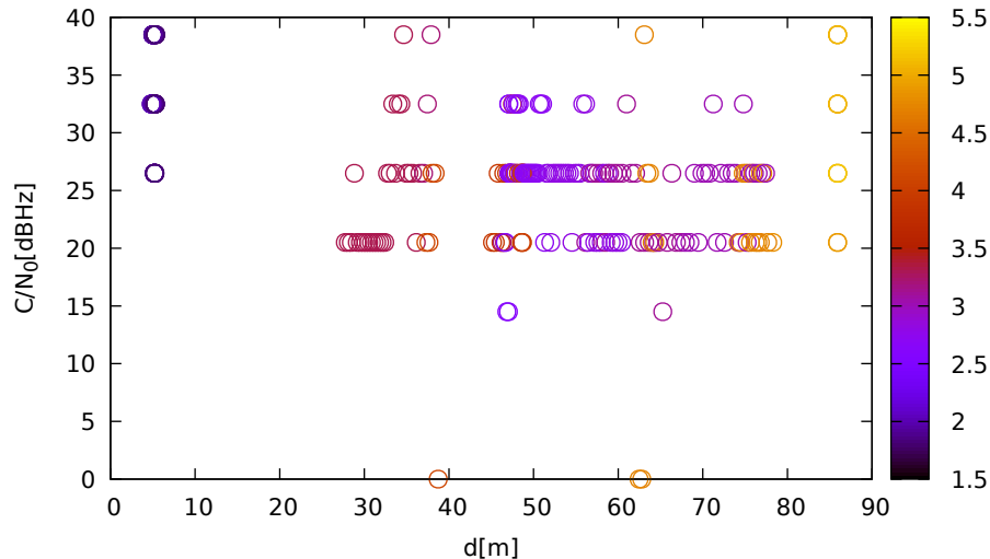
C/N 0 vs distance (LeicaGS15 at C 3 for R15 at L1)
