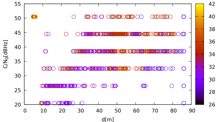
C/N 0 vs distance (LeicaGS15 at C 3 for R21 at L1)
