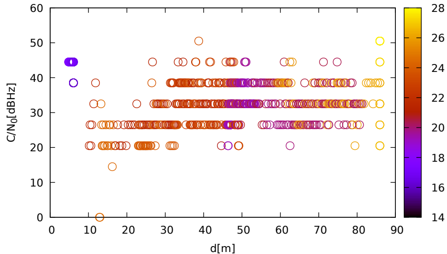
C/N 0 vs distance (LeicaGS15 at C 3 for R23 at L1)
