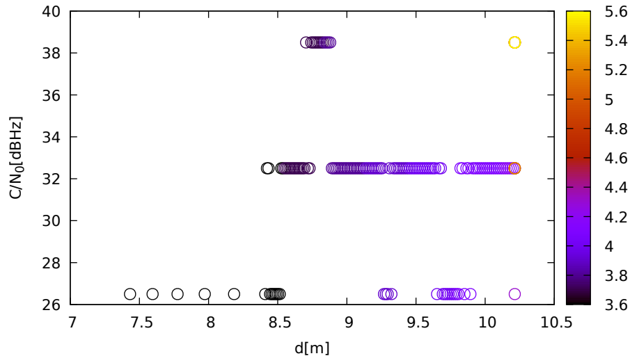
C/N 0 vs distance (LeicaGS18 at C 3 for E02 at L1)
