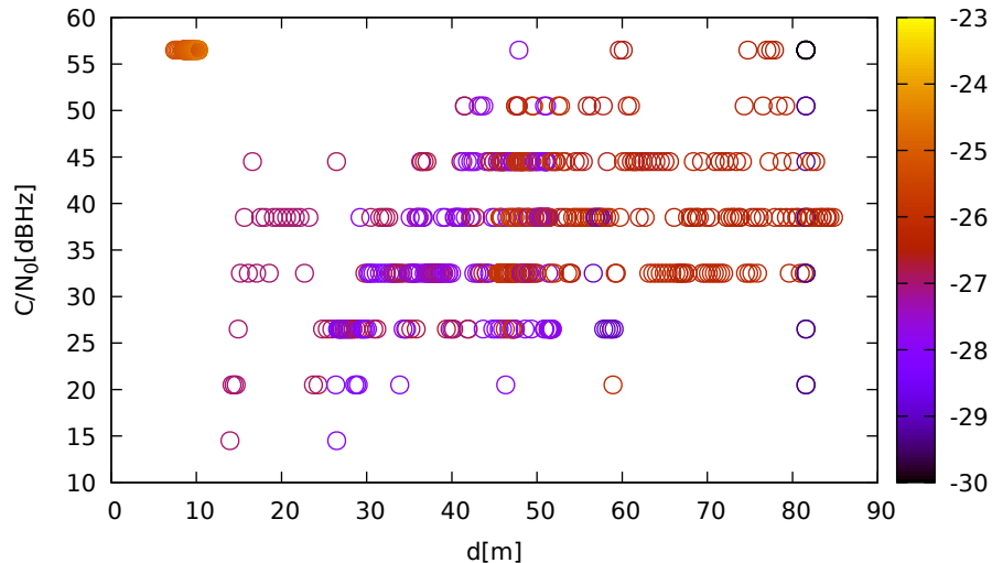
C/N 0 vs distance (LeicaGS18 at C 3 for E04 at L1)
