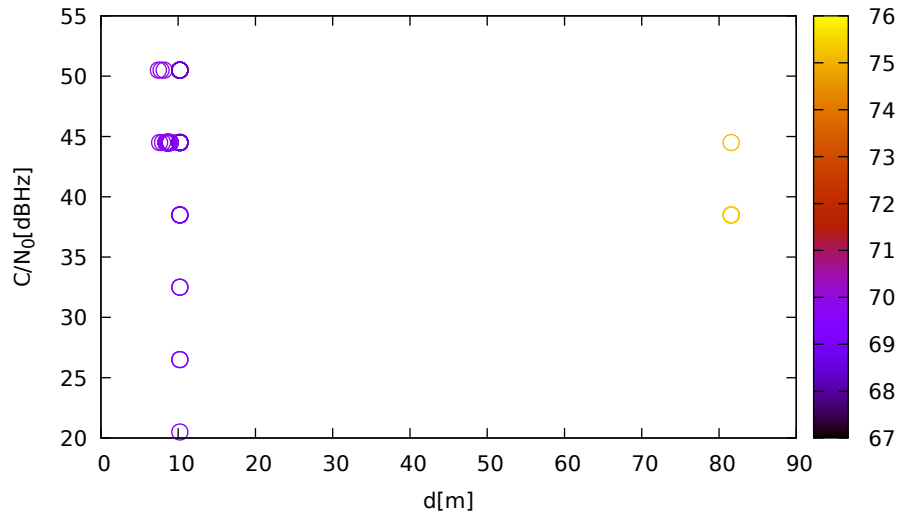
C/N 0 vs distance (LeicaGS18 at C 3 for E05 at L1)
