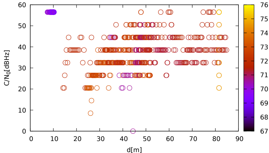
C/N 0 vs distance (LeicaGS18 at C 3 for E09 at L1)
