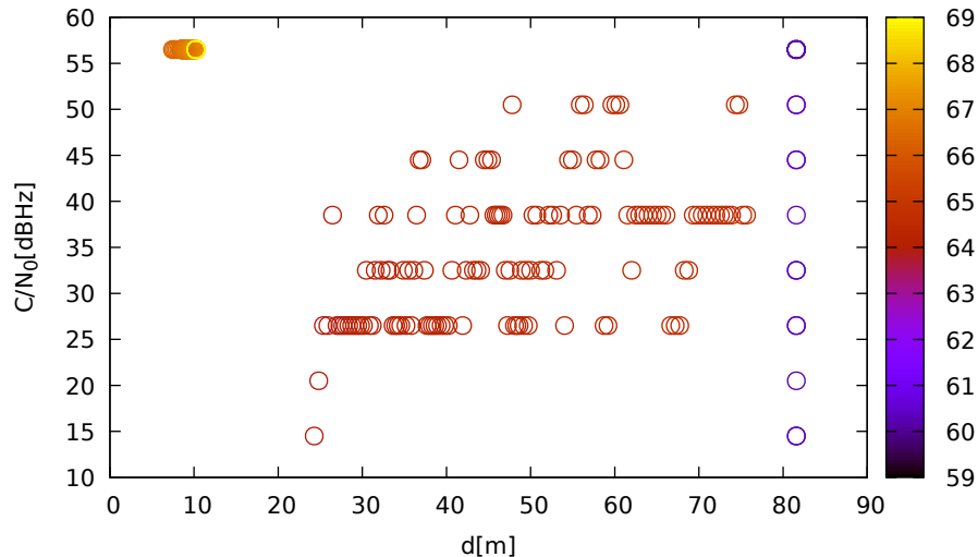
C/N 0 vs distance (LeicaGS18 at C 3 for E11 at L1)
