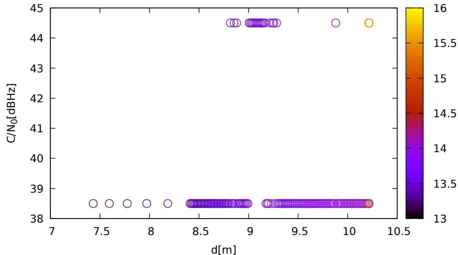
C/N 0 vs distance (LeicaGS18 at C 3 for E12 at L1)
