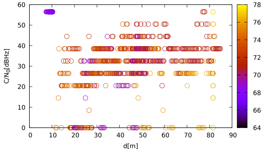
C/N 0 vs distance (LeicaGS18 at C 3 for G01 at L1)
