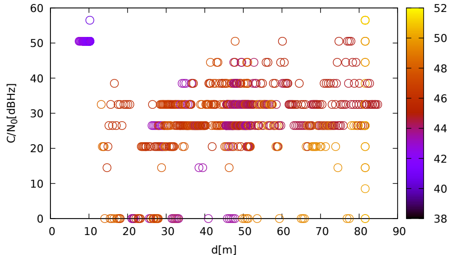
C/N 0 vs distance (LeicaGS18 at C 3 for G03 at L1)
