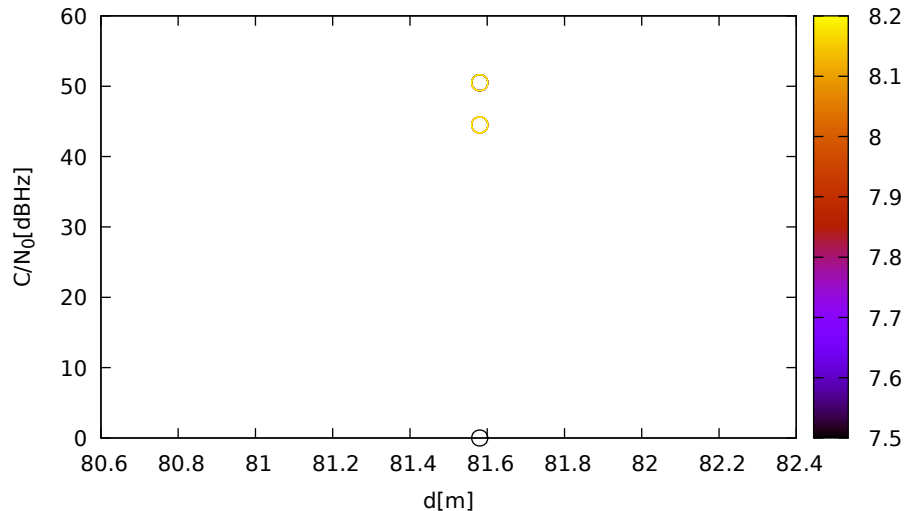
C/N 0 vs distance (LeicaGS18 at C 3 for G04 at L1)
