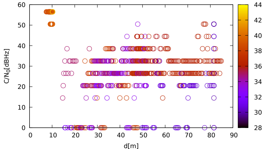
C/N 0 vs distance (LeicaGS18 at C 3 for G08 at L1)
