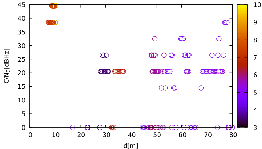
C/N 0 vs distance (LeicaGS18 at C 3 for G10 at L1)
