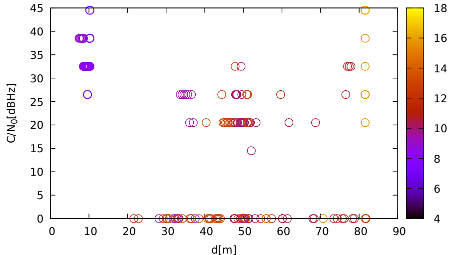
C/N 0 vs distance (LeicaGS18 at C 3 for G17 at L1)
