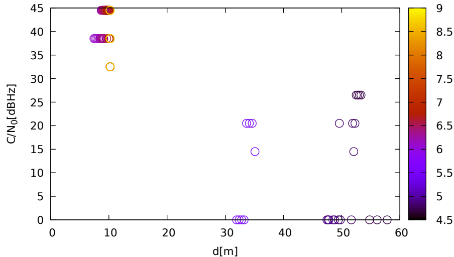
C/N 0 vs distance (LeicaGS18 at C 3 for G21 at L1)
