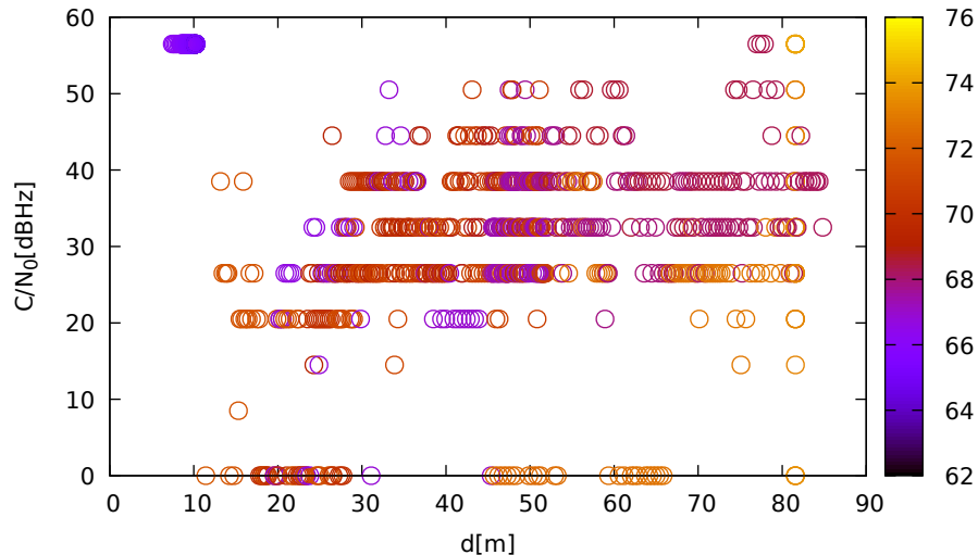
C/N 0 vs distance (LeicaGS18 at C 3 for G22 at L1)
