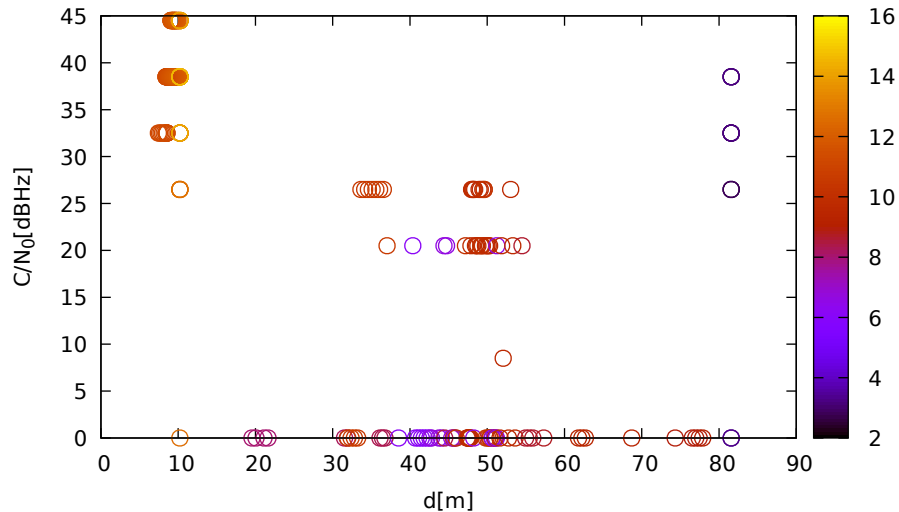
C/N 0 vs distance (LeicaGS18 at C 3 for G27 at L1)
