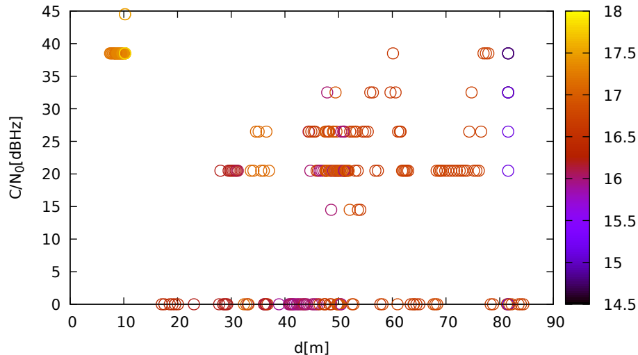
C/N 0 vs distance (LeicaGS18 at C 3 for G28 at L1)
