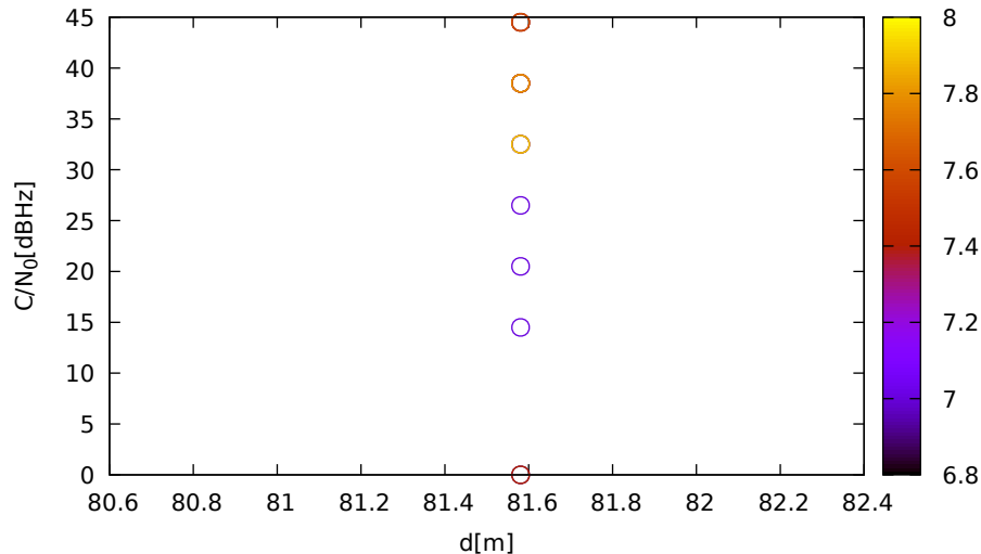
C/N 0 vs distance (LeicaGS18 at C 3 for G31 at L1)
