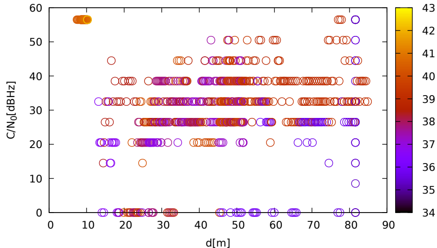
C/N 0 vs distance (LeicaGS18 at C 3 for G32 at L1)
