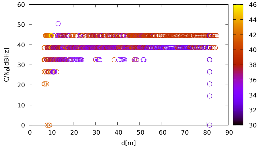
C/N 0 vs distance (LeicaGS18 at C 3 for R06 at L1)
