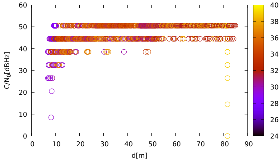
C/N 0 vs distance (LeicaGS18 at C 3 for R08 at L1)
