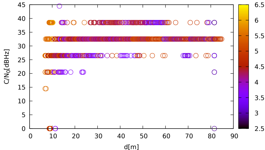
C/N 0 vs distance (LeicaGS18 at C 3 for R14 at L1)
