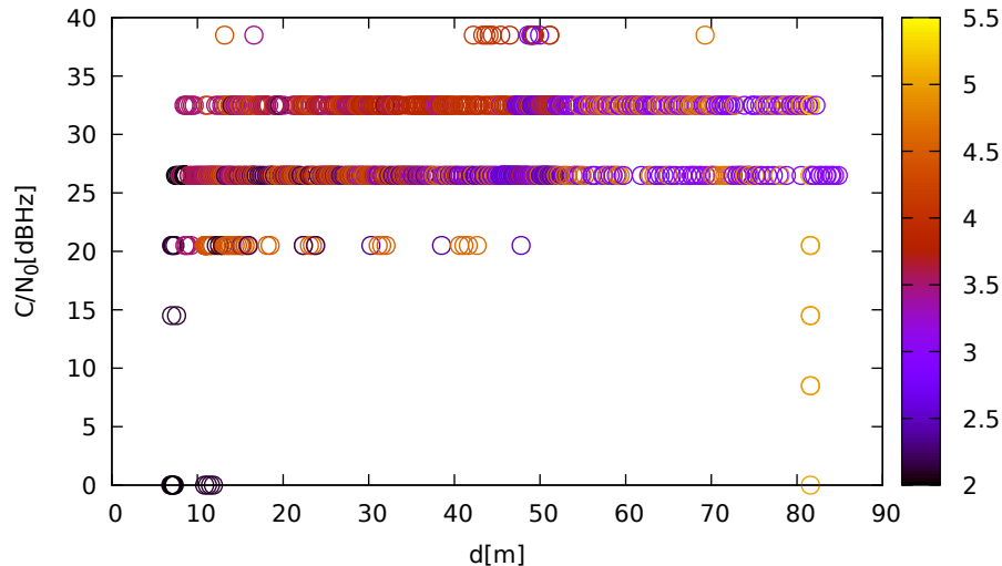
C/N 0 vs distance (LeicaGS18 at C 3 for R15 at L1)
