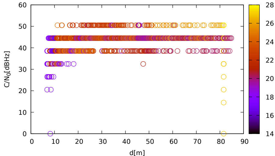
C/N 0 vs distance (LeicaGS18 at C 3 for R23 at L1)
