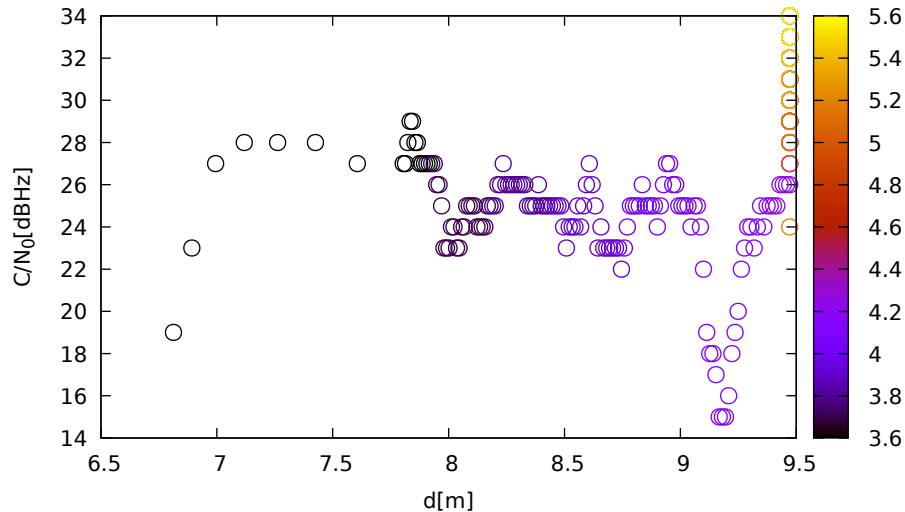
C/N 0 vs distance (ublox9 at C 3 for E02 at L1)
