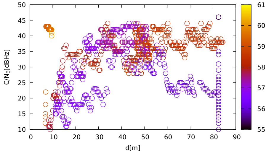
C/N 0 vs distance (ublox9 at C 3 for E04 at L1)
