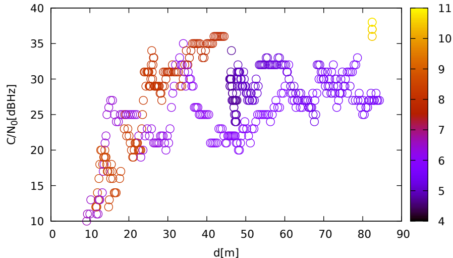
C/N 0 vs distance (ublox9 at C 3 for E05 at L1)
