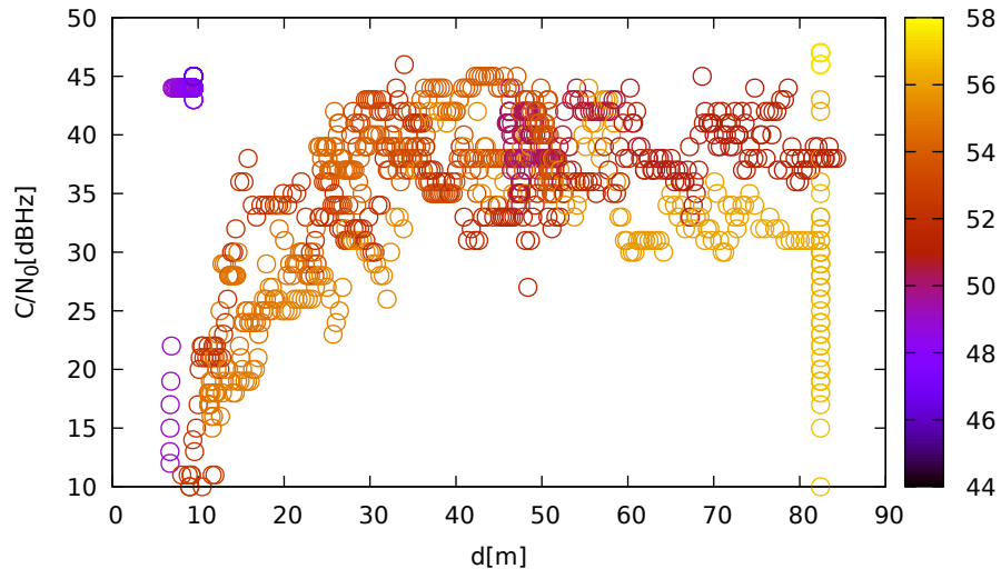
C/N 0 vs distance (ublox9 at C 3 for E09 at L1)
