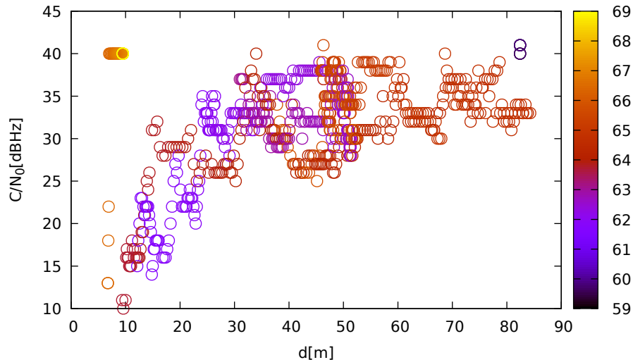
C/N 0 vs distance (ublox9 at C 3 for E11 at L1)
