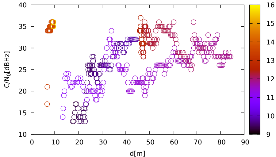
C/N 0 vs distance (ublox9 at C 3 for E12 at L1)
