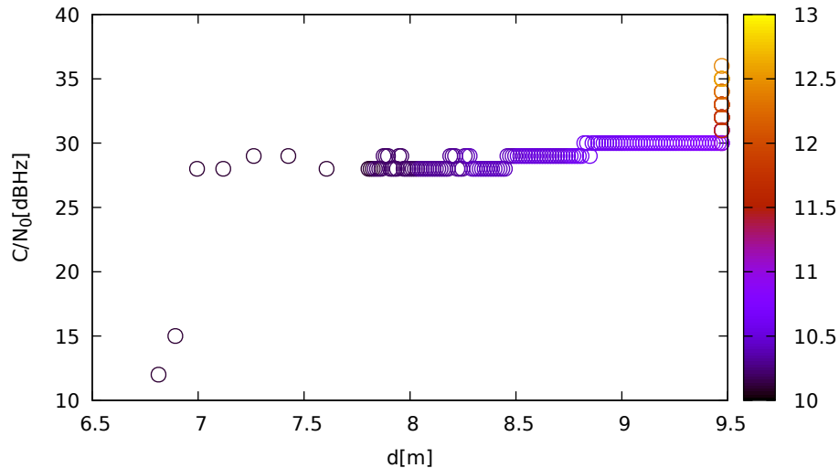
C/N 0 vs distance (ublox9 at C 3 for E19 at L1)
