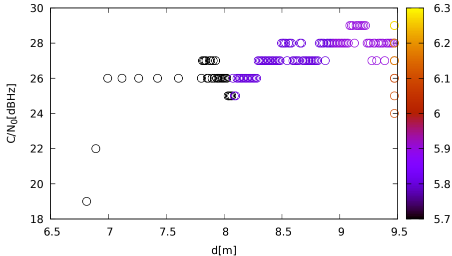
C/N 0 vs distance (ublox9 at C 3 for E30 at L1)
