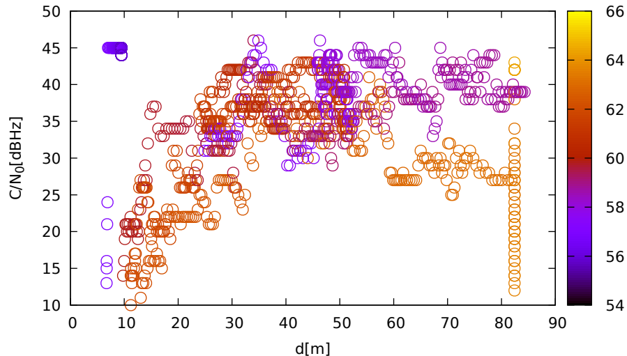
C/N 0 vs distance (ublox9 at C 3 for E36 at L1)
