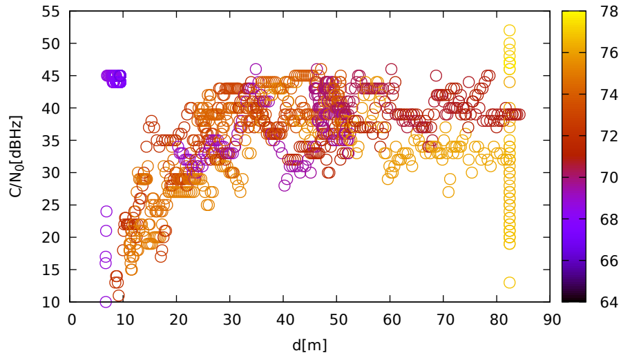
C/N 0 vs distance (ublox9 at C 3 for G01 at L1)
