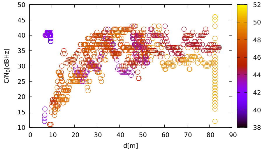
C/N 0 vs distance (ublox9 at C 3 for G03 at L1)
