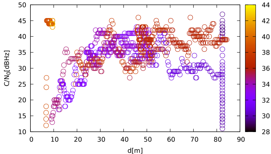
C/N 0 vs distance (ublox9 at C 3 for G08 at L1)
