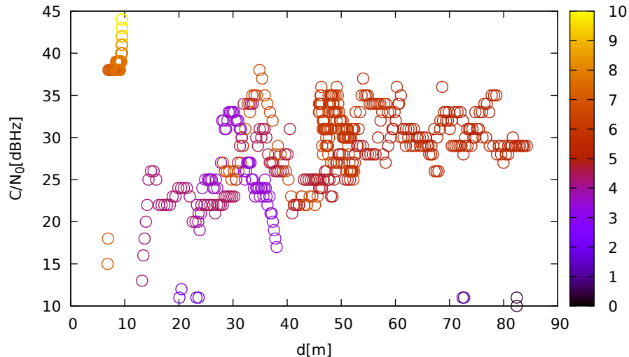
C/N 0 vs distance (ublox9 at C 3 for G10 at L1)
