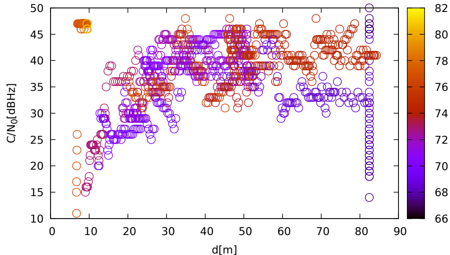
C/N 0 vs distance (ublox9 at C 3 for G11 at L1)
