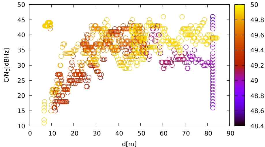
C/N_0 vs distance (ublox9 at C_3 for G14 at L1)
