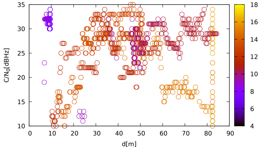
C/N 0 vs distance (ublox9 at C 3 for G17 at L1)
