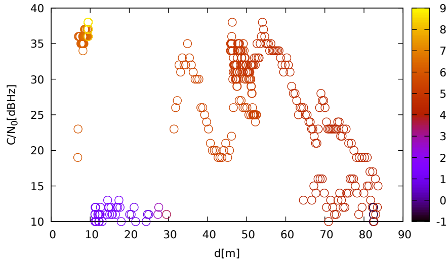
C/N 0 vs distance (ublox9 at C 3 for G21 at L1)
