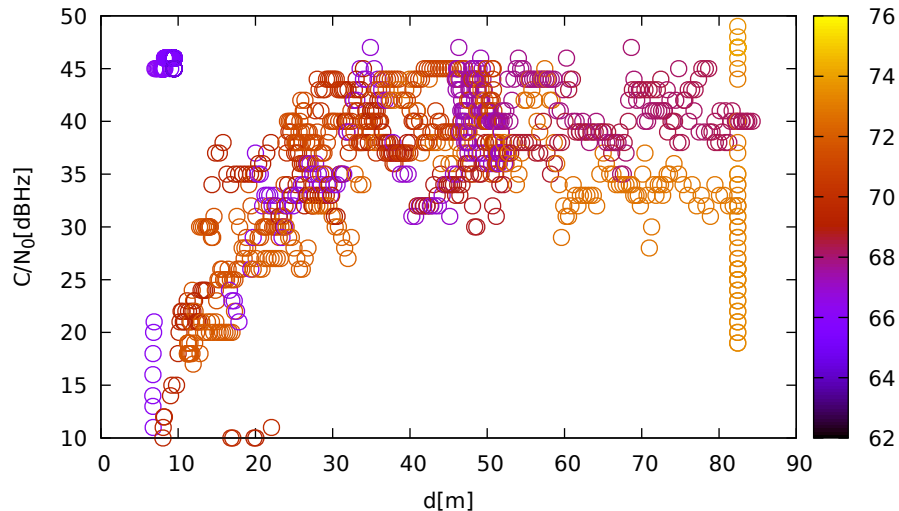
C/N 0 vs distance (ublox9 at C 3 for G22 at L1)
