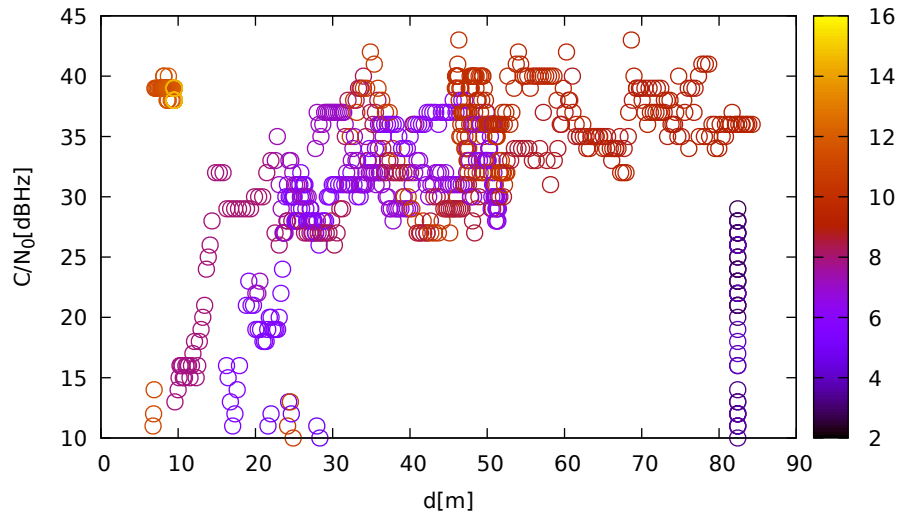
C/N 0 vs distance (ublox9 at C 3 for G27 at L1)
