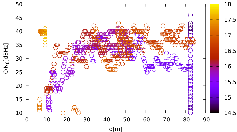
C/N 0 vs distance (ublox9 at C 3 for G28 at L1)
