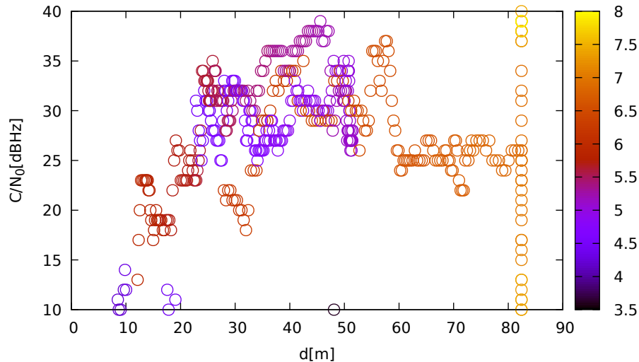
C/N 0 vs distance (ublox9 at C 3 for G31 at L1)
